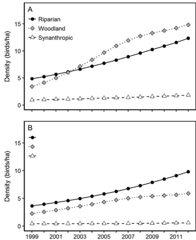
Figure 3. Long-term trends in the density (birds/ha) of the lower Putah Creek breeding bird community by habitat association group. A) Including all species. B) Excluding secondary cavity nesters.
